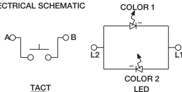
ELECTRICAL SCHEMATIC
