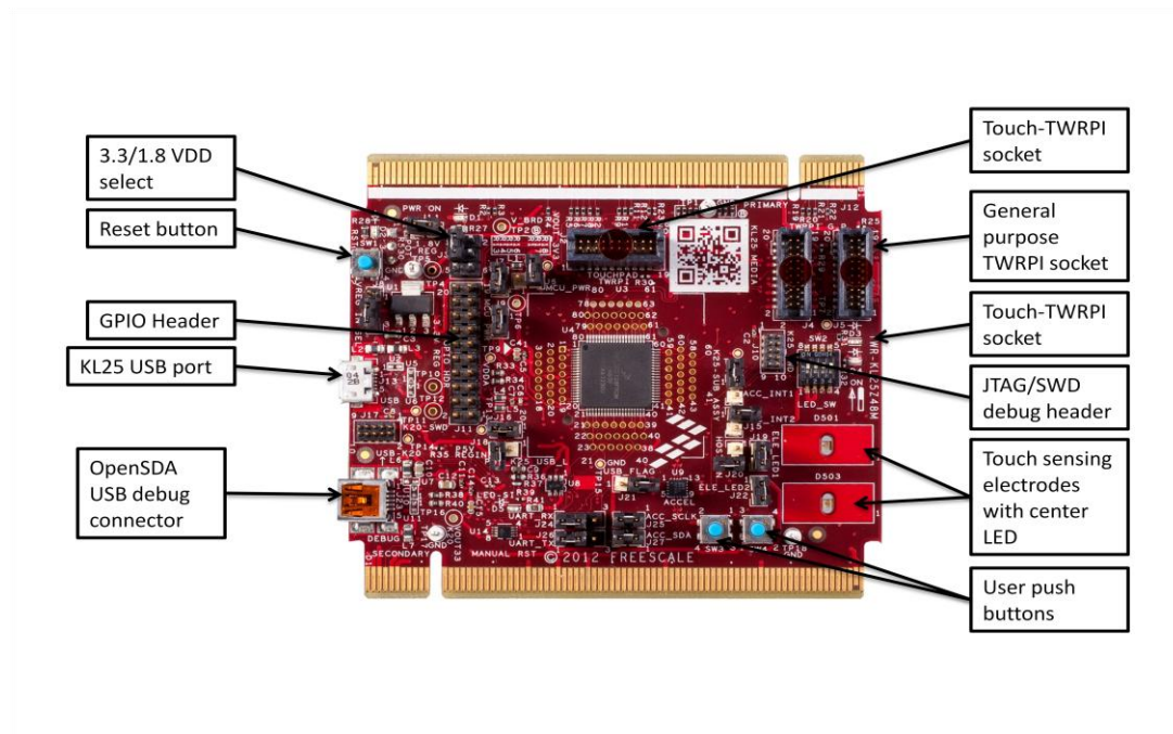
Figure 2 Top side of TWR-KL25Z module
