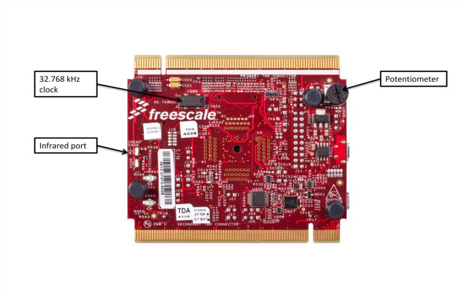
Figure 3 Bottom side of TWR-KL25Z module
