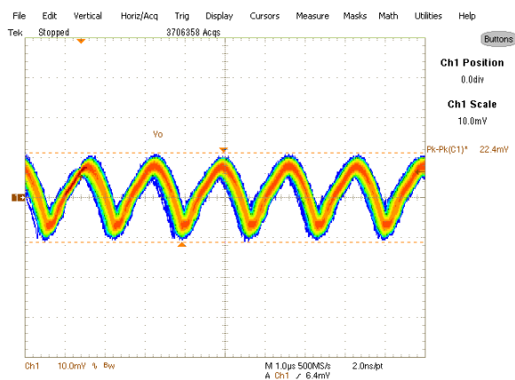
Fig. 10: Output Voltage Ripple, 12A load Ch 1 : V out
