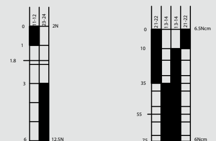
Slow-action contact Snap-action contact
