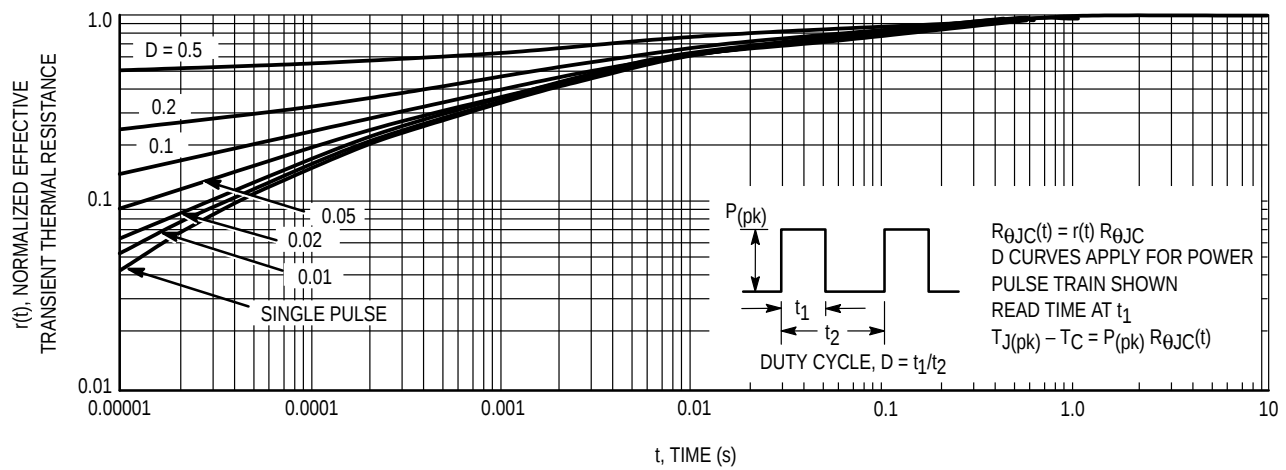
Figure 13. Thermal Response
