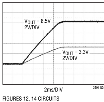
Soft Start-Up
