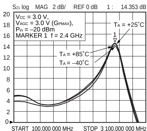
S 21 —FREQUENCY
