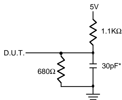
Figure 1. Output Load
