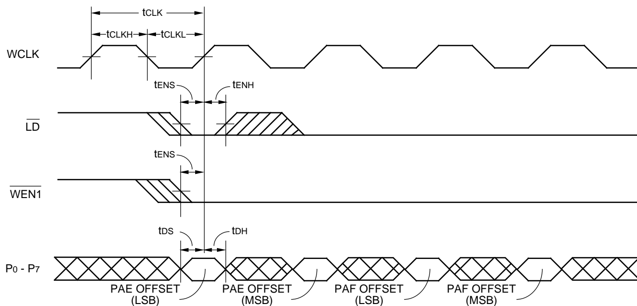
Figure 11. Programmable Empty Flag Timing
