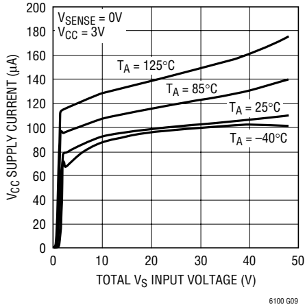
V CC Supply Current vs V S Input Voltage
