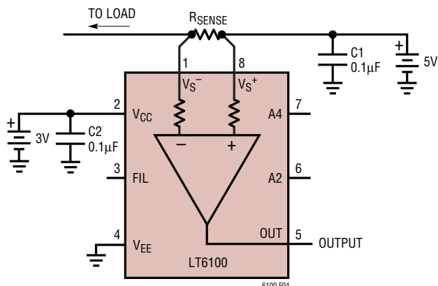
Figure 4. LT6100 Load Current Monitor
