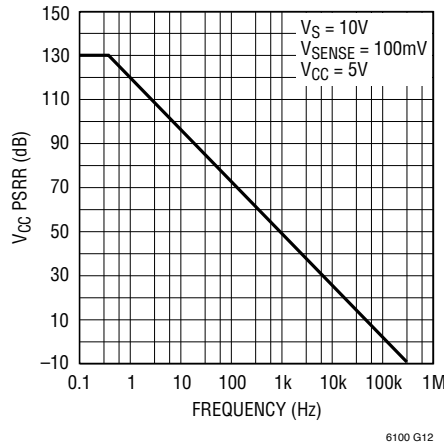
V CC PSRR vs Frequency
