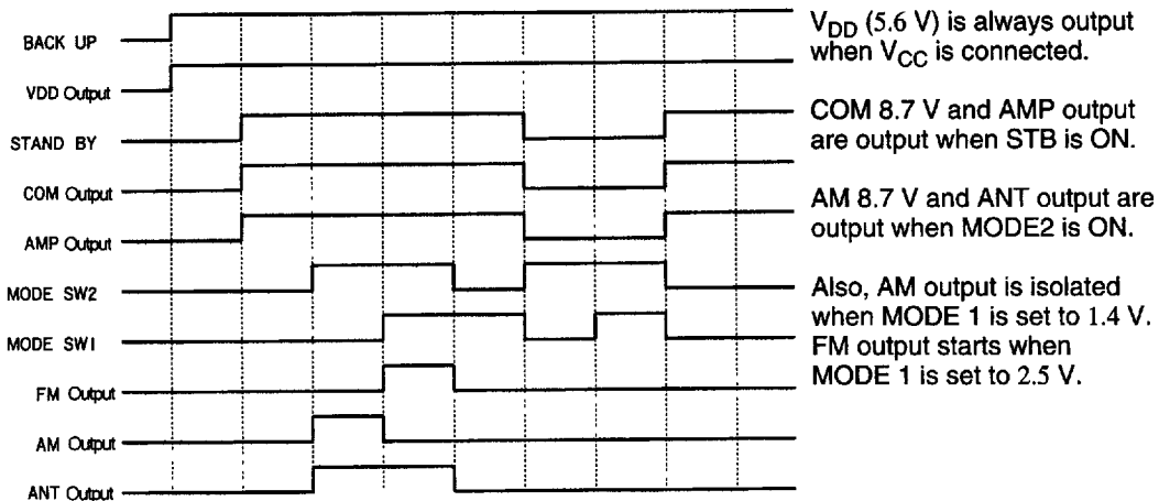
Figure 5 Timing chart
