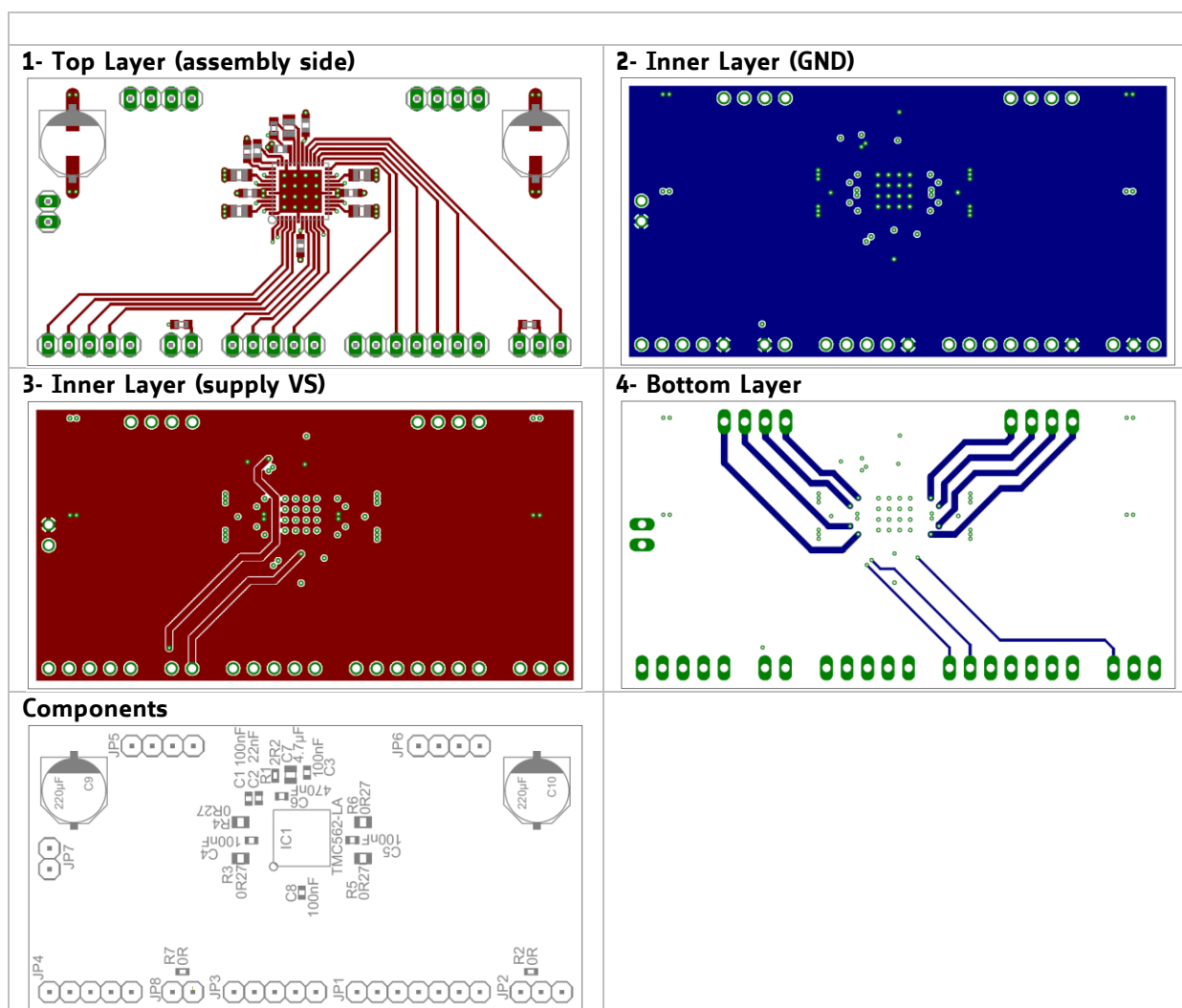
Figure 16.1 Layout example
