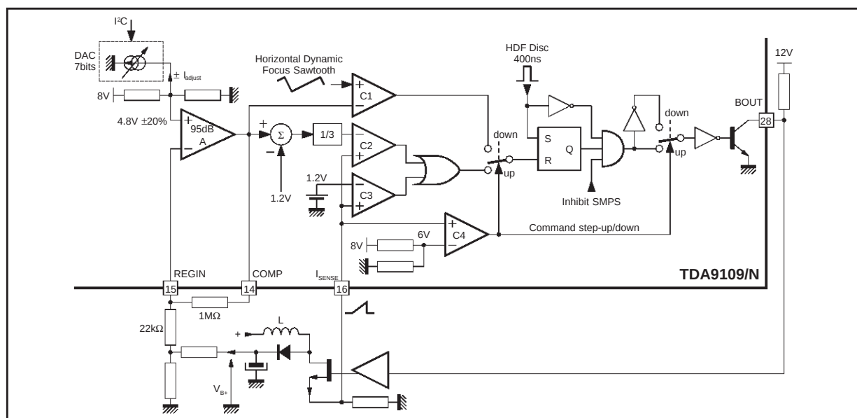
Figure 18 : DC/DC Converter
