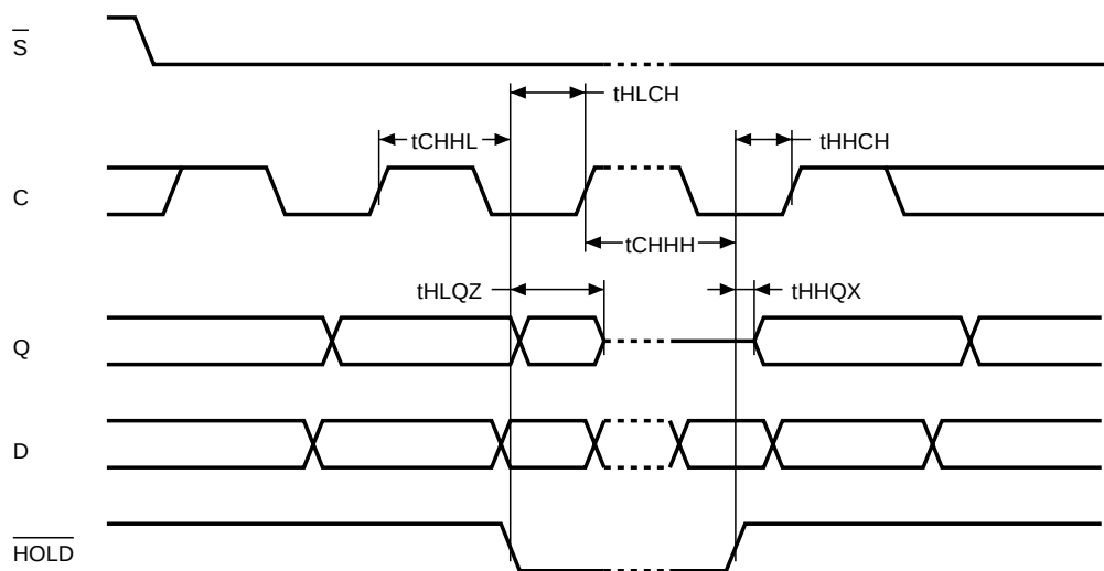
Figure 18. Hold Timing
