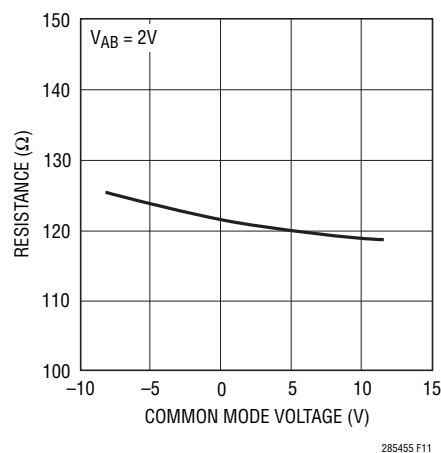
Figure 11. Typical Resistance of the Enabled Terminator vs Voltage on B Pin
