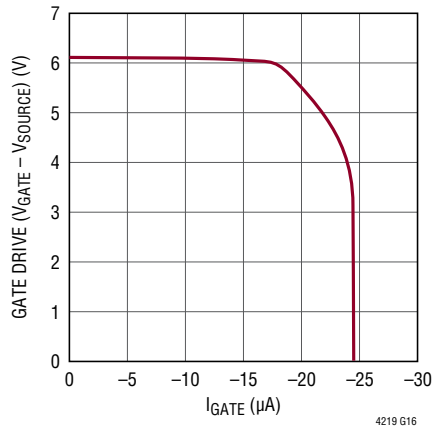
Gate Pull-Up Current vs Gate Drive
