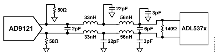
Figure 74. DAC Modulator Interface with Fifth-Order, Low-Pass Filter
