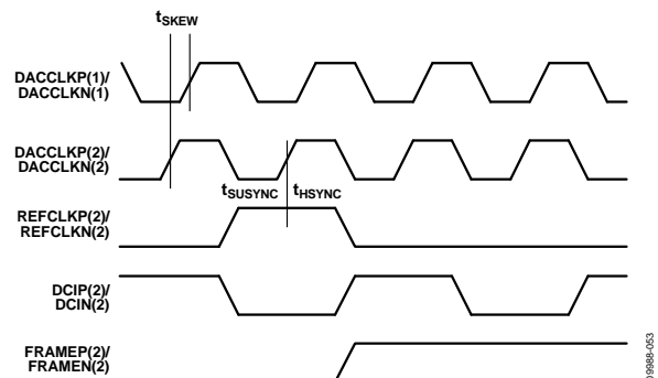
Figure 85. FIFO Rate Synchronization Signal Timing Requirements, 2× Interpolation
