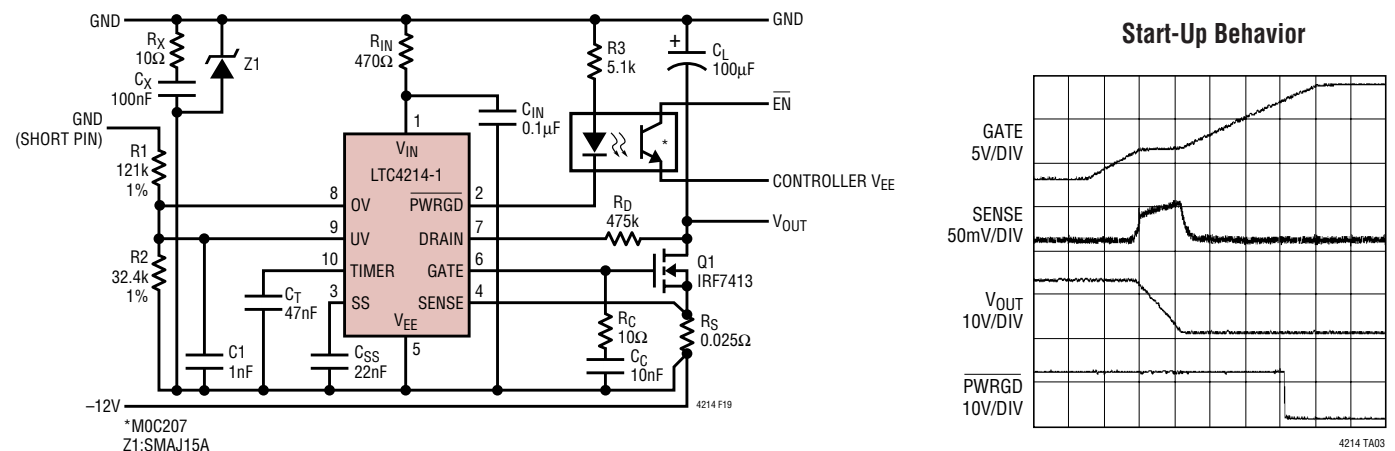
Figure 19. -12V/2A Hot Swap Controller
