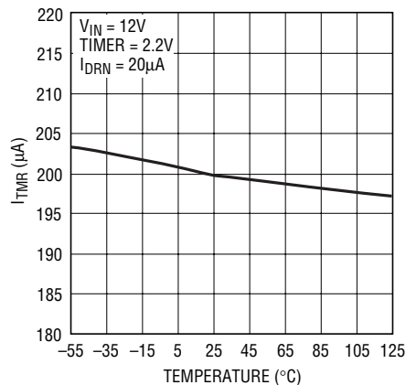
I_{TMR} (Circuit Breaker, I_{DRN} = 20\mu A , Sourcing) vs Temperature
