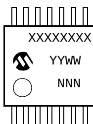
14-Lead TSSOP (4.4mm) (MCP604 Only)
