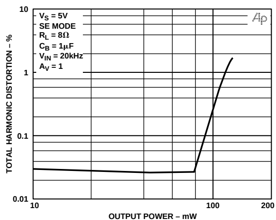
Figure 11. SE Out THD + N vs. Output Power at 20 kHz
