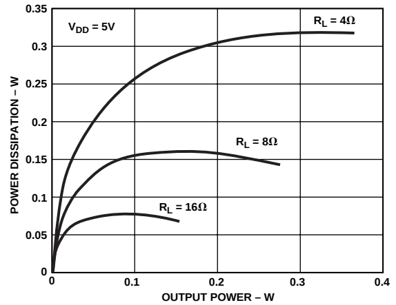
Figure 14. Power Dissipation vs. Single-Ended Output Power ( V_{DD} = 5 V)
