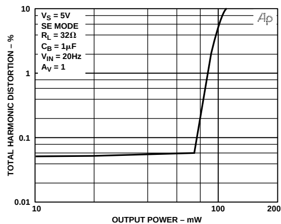
Figure 10. SE Out THD + N vs. Output Power at 20 Hz
