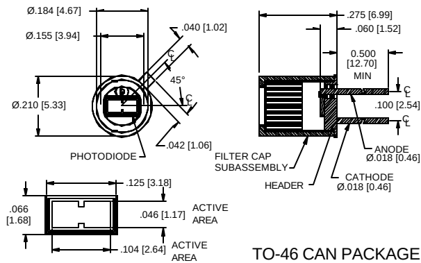
TO-46 CAN PACKAGE
