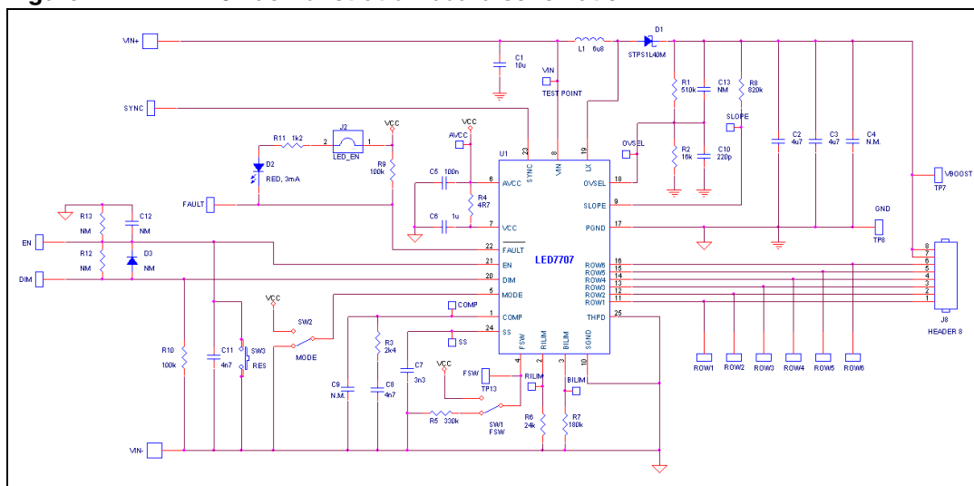
Figure 24. LED7707 demonstration board schematic
