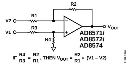
Figure 64. Using the AD8571/AD8572/AD8574 as a Difference Amplifier
