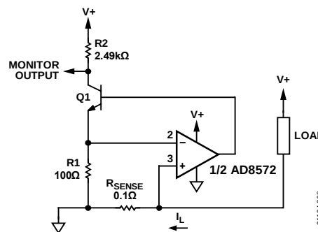
Figure 68. Low-Side Load Current Monitor
