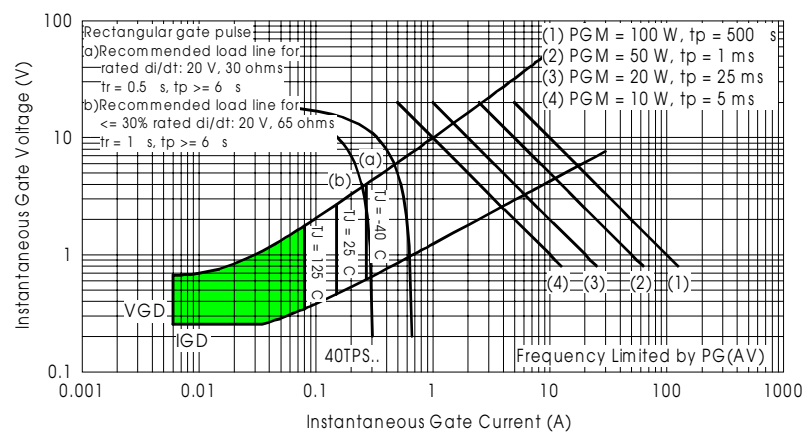
Fig. 8 - Gate Characteristics
