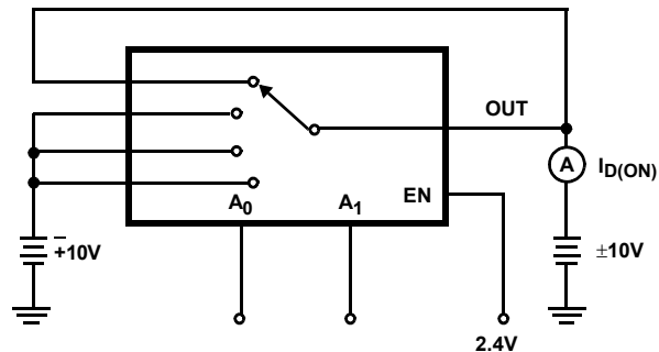
FIGURE 2D. I_{D(ON)} TEST CIRCUIT (NOTE 12)
