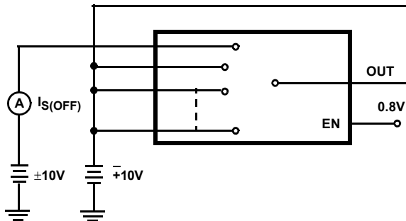
FIGURE 2C. I_{S(OFF)} TEST CIRCUIT (NOTE 12)
