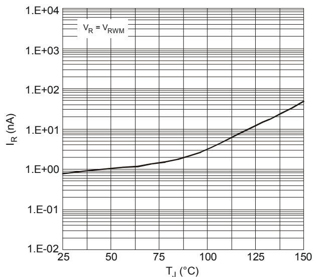
Figure 8 Leakage Current vs. Junction Temperature (typical values)
