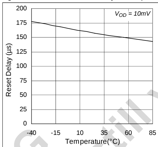
Figure 4. Power Down Reset Delay vs. Temp.
