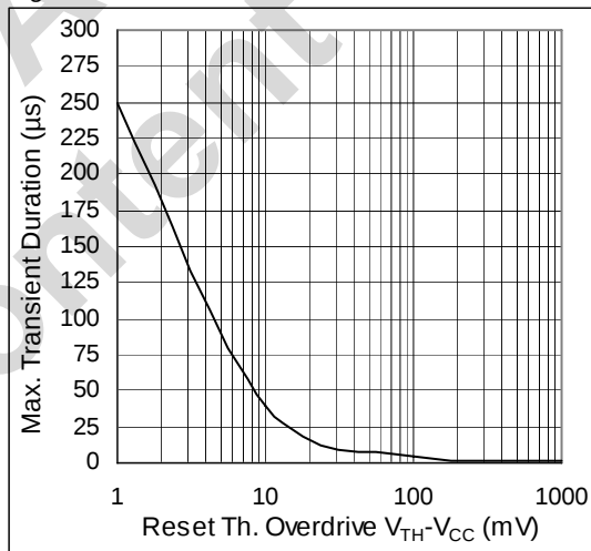
Figure 6. Max. Trans. Duration vs. Reset Th.
