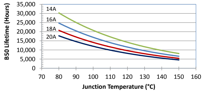
CBT120-UV B50 Lifetime
