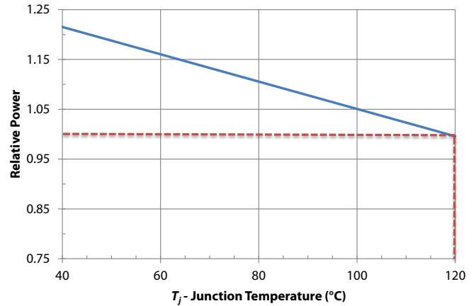
Relative Power vs Junction Temperature ( T_j ) I_f = 18\text{ A} , normalized to 120^\circ\text{C}
