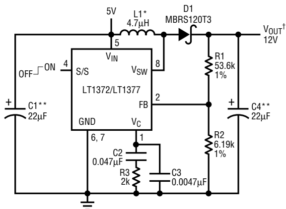
5V-to-12V Boost Converter
