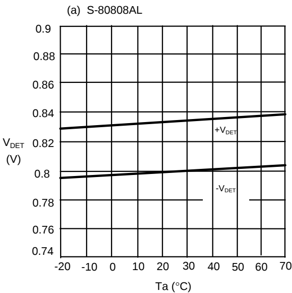
(1) Detection voltage ( V_{DET} ) - Temperature ( T_a )
