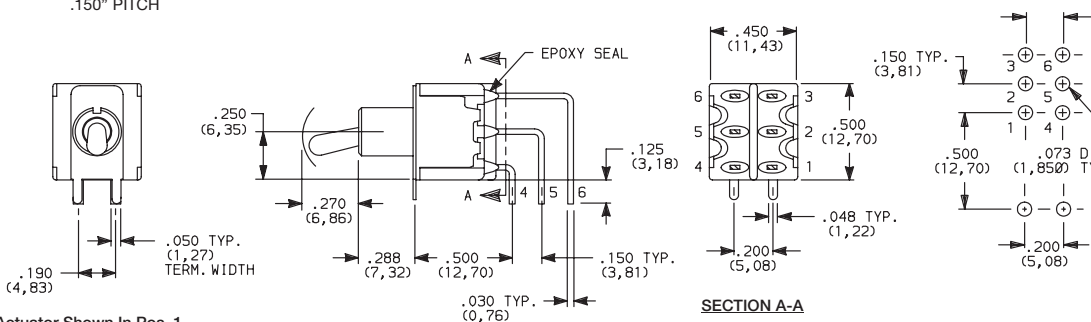
7201MD9AV2BE Vertical Actuation DPDT
