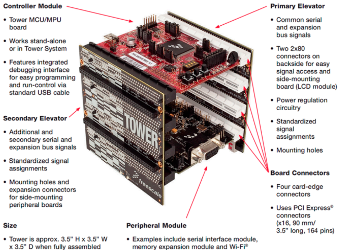
Figure 1-2. Callouts on front side of the TWR-P1025
