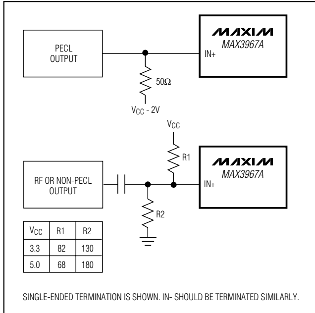
Figure 3. Input Terminations
