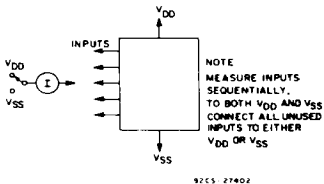
Fig. 12 — Input current.
