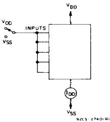
Fig. 10 — Quiescent device current.
