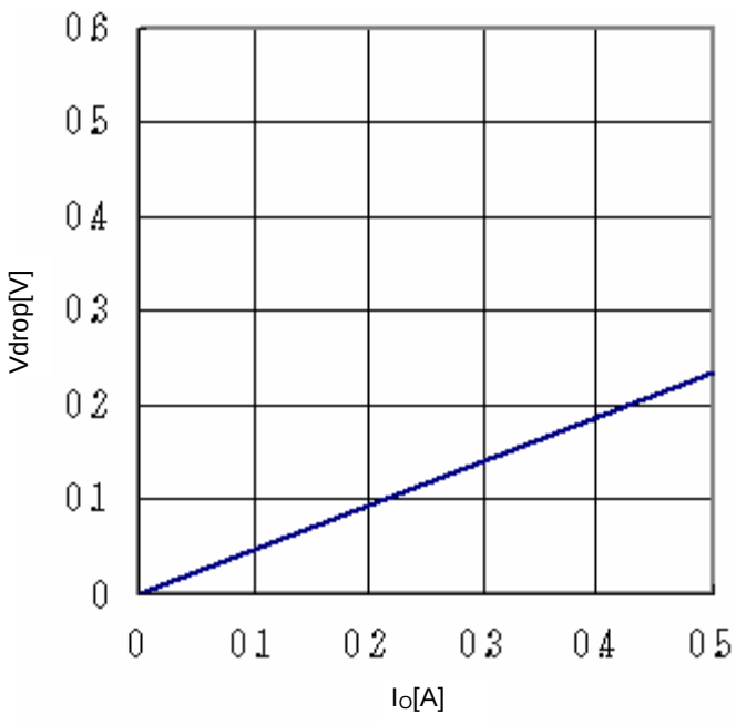
Fig.26 Minimum dropout Voltage 6 (V CC =12V、Ta=25°C)
