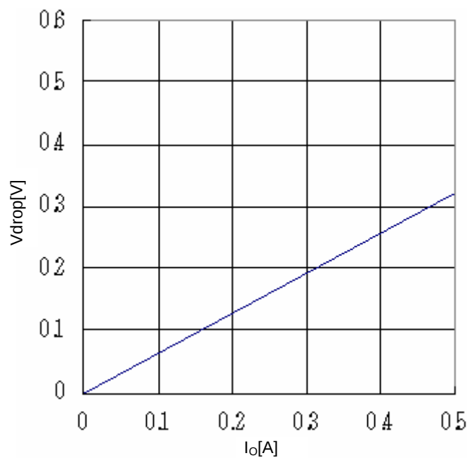
Fig.23 Minimum dropout Voltage 3 (V CC =6V、Ta=25°C)
