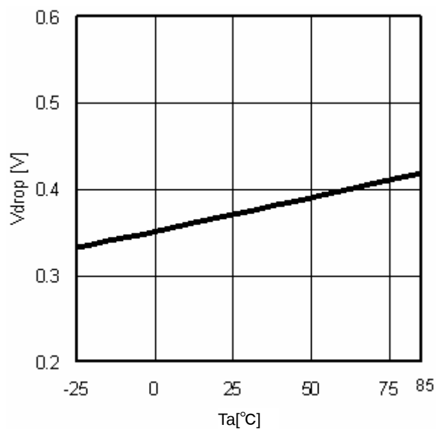
Fig.18 Minimum dropout Voltage1 ( V_{CC}=5\text{V} , I_O=-0.5\text{A} )
