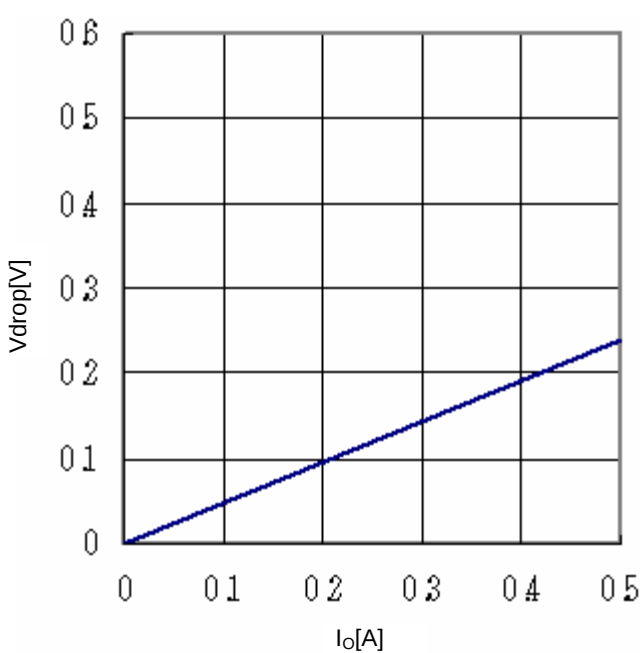
Fig.25 Minimum dropout Voltage 5 (V CC =10V、Ta=25°C)
