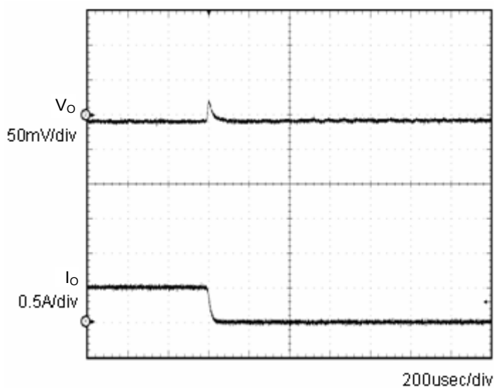
Fig.4 Transient Response (0.5→0A) C_o=1\mu\text{F}
