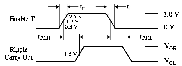
Figure 2. Switching Waveform
