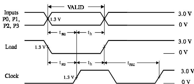
Figure 3. Switching Waveform
