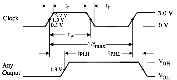
Figure 1. Switching Waveform
