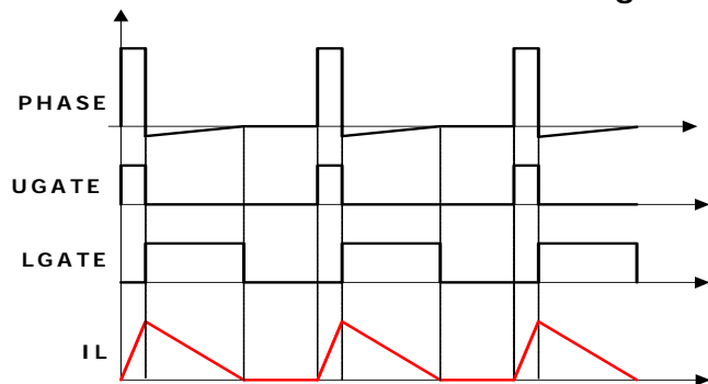
FIGURE 8. DIODE EMULATION
