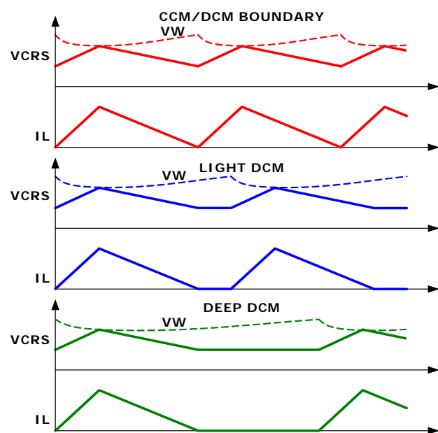
FIGURE 9. PERIOD STRETCHING
