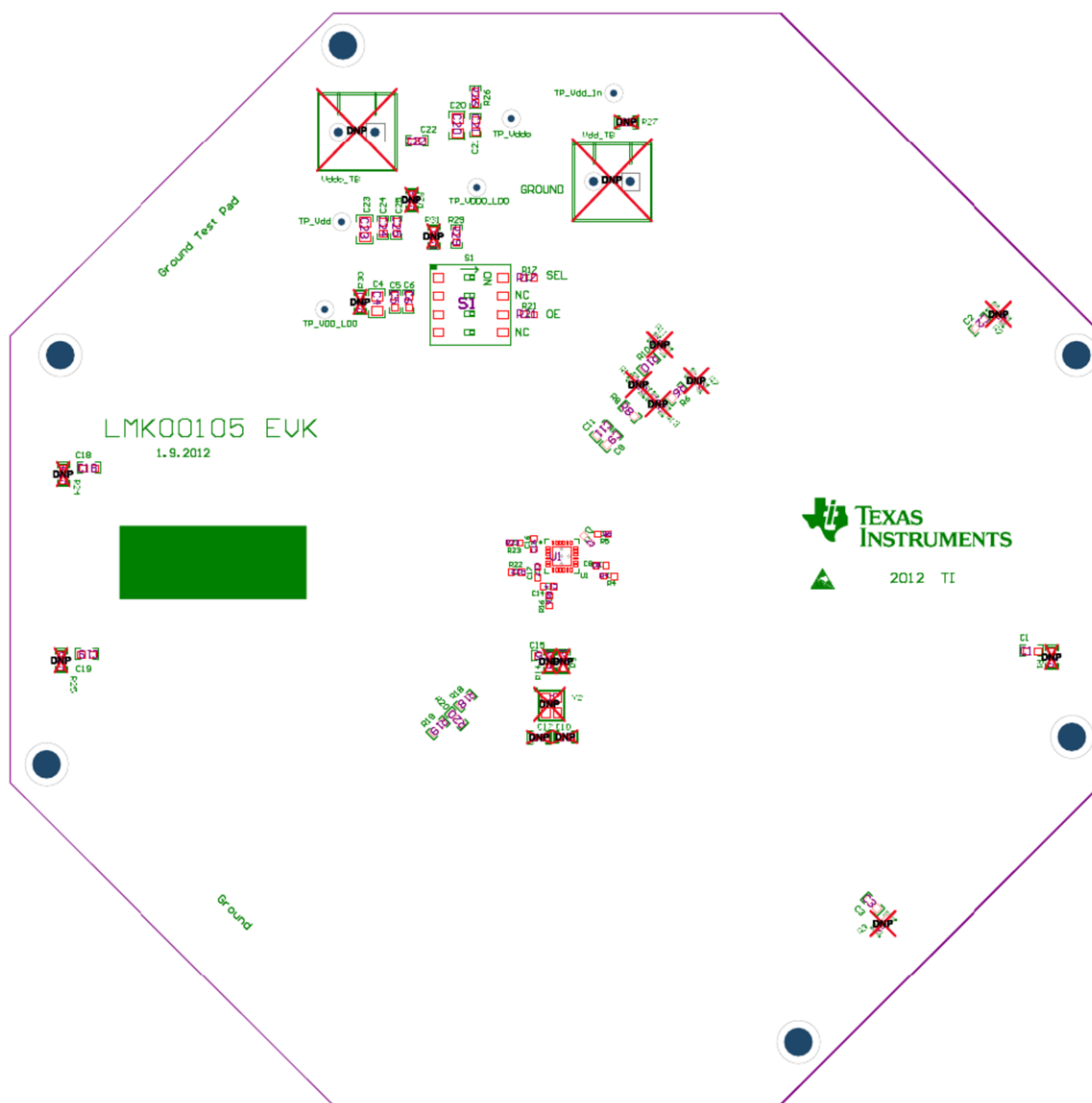
Figure 4. PCB Top
