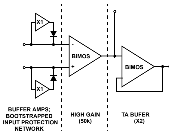
FIGURE 1. FUNCTIONAL DIAGRAM
