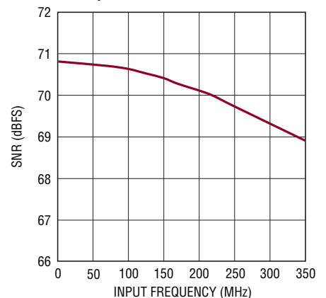
LTC2171-12: SNR vs Input Frequency, -1\text{dBFS} , 2\text{V} Range, 40\text{Mpsps}
