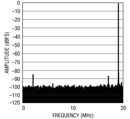
LTC2171-12: 8k Point FFT, f_{IN} = 139\text{MHz} , -1\text{dBFS} , 40\text{Mpsps}
