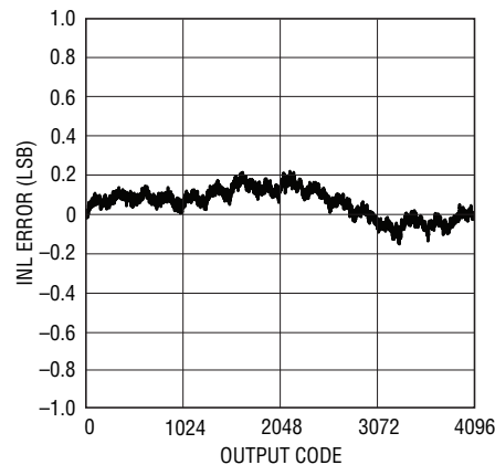
LTC2171-12: Integral Nonlinearity (INL)
