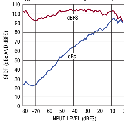
LTC2171-12: SFDR vs Input Level, f_{IN} = 70\text{MHz} , 2\text{V} Range, 40\text{Mpsps}
