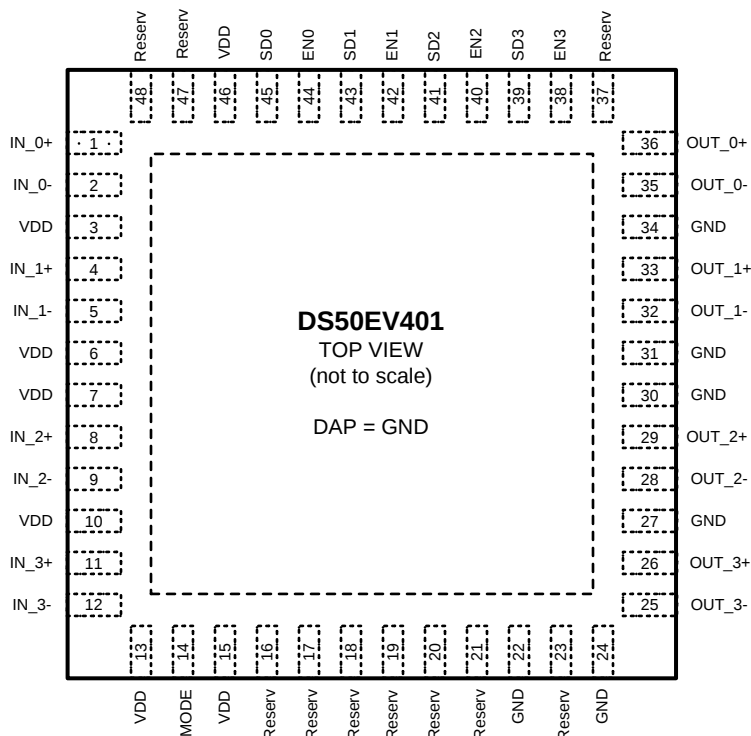
Figure 1. TOP VIEW — Not to scale
