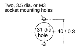
Mounting Holes
