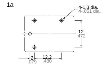
PC board pattern (Copper-side view)
