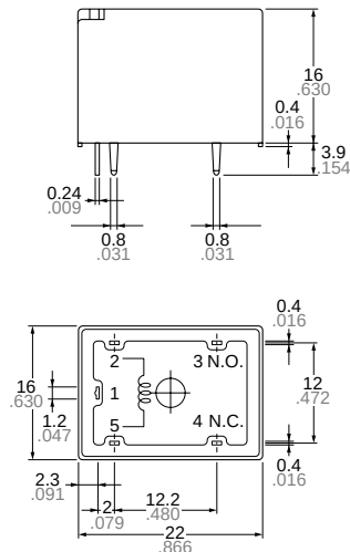
Schematic (Bottom view)
