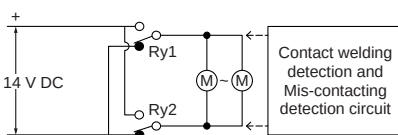
Circuit
