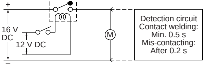
Circuit
