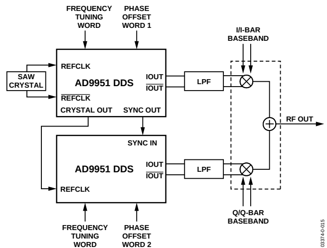
Figure 27. Two AD9951s Synchronized to Provide I and Q Carriers with Independent Phase Offsets for Nulling
