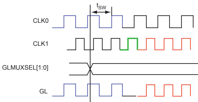
Figure 2-26 • NGMUX Waveform
