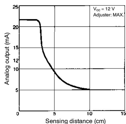
E32-TC200E with E3XA-CC4A analog output amplifier
