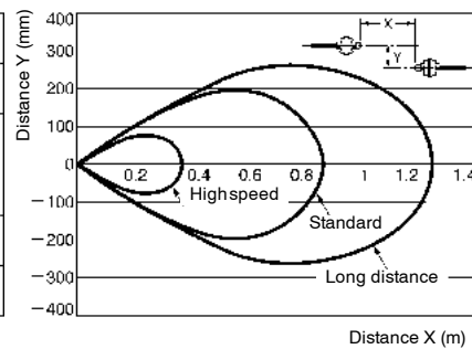
E32-T11R with E3X-DAN amplifier (Through-beam)
