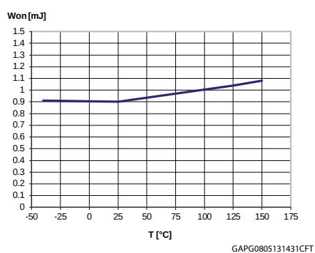
Figure 29: W_{on} vs. T_{case}
