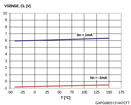
Figure 33: V_{sense\_clamp} vs. T_{case}
