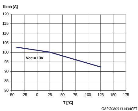
Figure 31: I_{limH} vs. T_{case}
