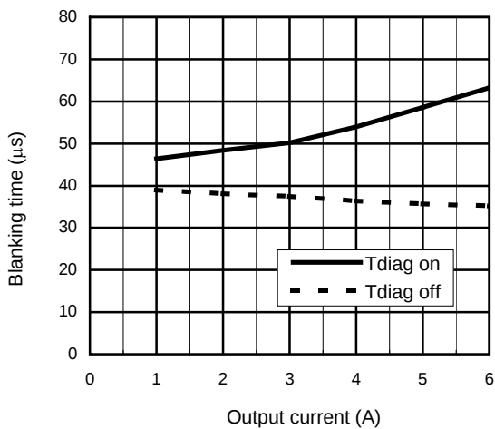
Figure 12 – Diagnosis Blanking time (μs) Vs Output current (A)
