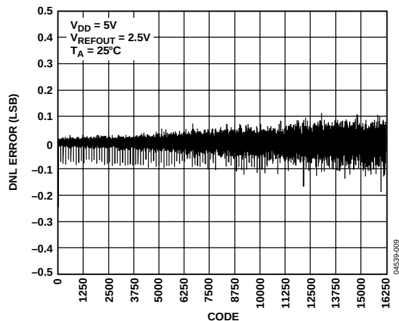
Figure 9. DNL—AD5640-2/AD5640-3
