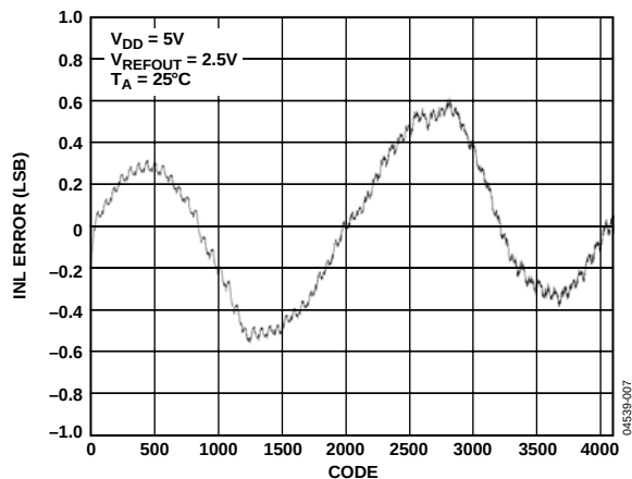
Figure 7. INL—AD5620-2/AD5620-3
