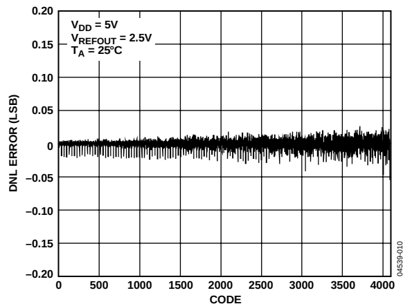
Figure 10. DNL—AD5620-2/AD5620-3
