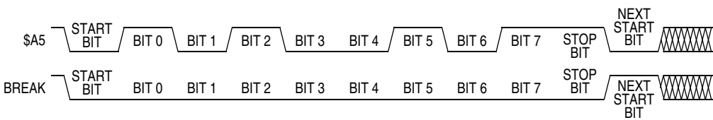
Figure 10-4. Sample Monitor Waveforms
