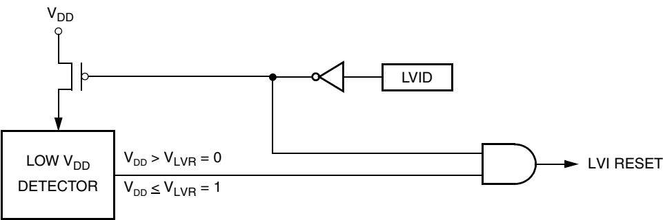
Figure 16-1. LVI Module Block Diagram
