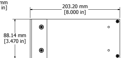
ASSEMBLT - VIEW FROM SIDE
