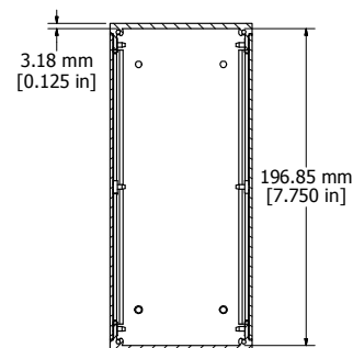
SECTION DD-DD
