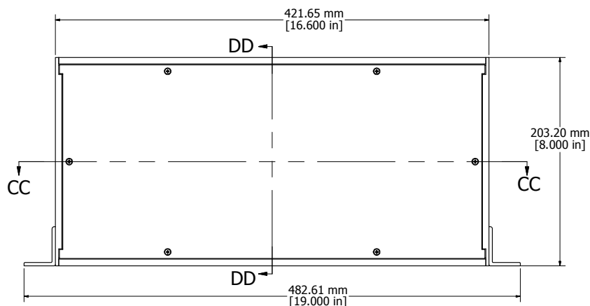
ASSEMBLY - VIEW FROM TOP
